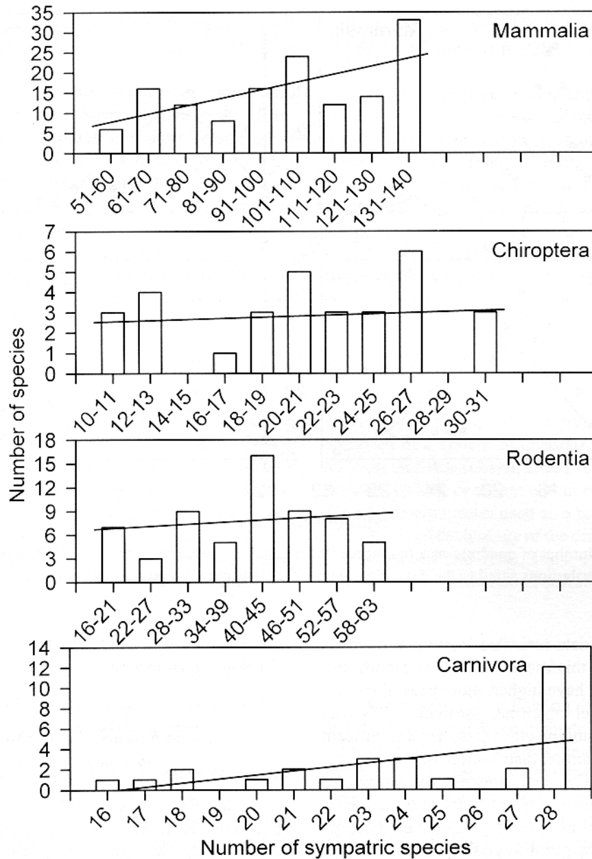
Figure 2. Number of species, as a function of the total number of species with which they are geographically sympatric.
